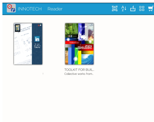
Shelf View
