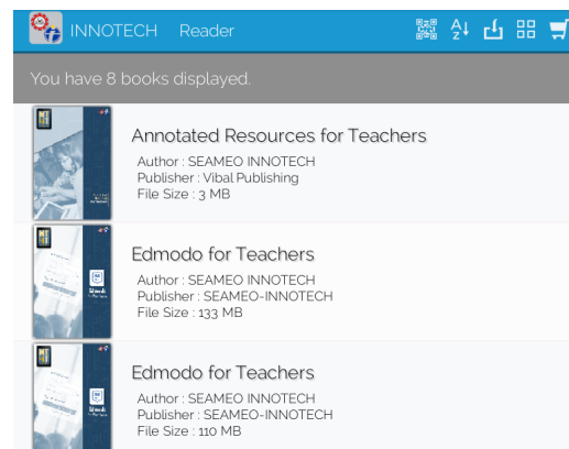
List View
